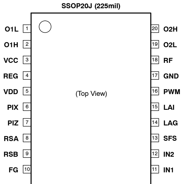
Figure 3. LV88561JA, LV88562JA, LV88563JA, LV88564JA Pin Assignment
