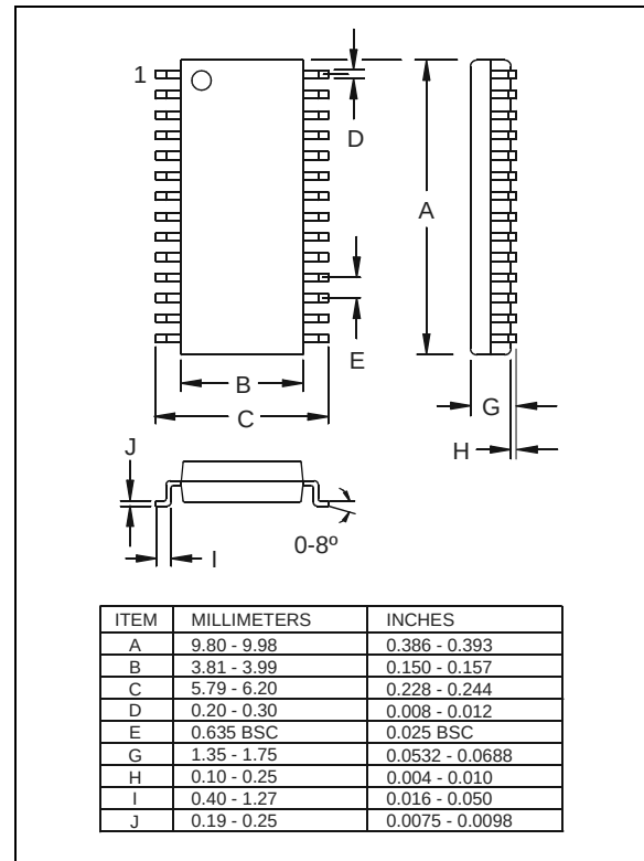
Figure 14. QSOB-28 package drawing
