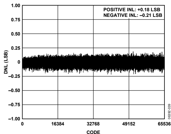
Figure 9. Differential Nonlinearity vs. Code, REF = 5\text{ V}
