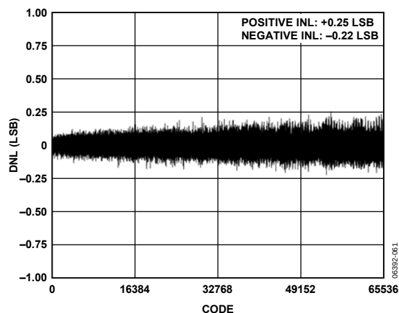
Figure 10. Differential Nonlinearity vs. Code, REF = 2.5\text{ V}
