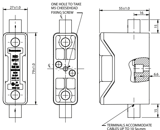
Front connected
