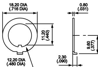
LOCKING RING 12mm (.472") Nickel plated U121 Matte black U12
