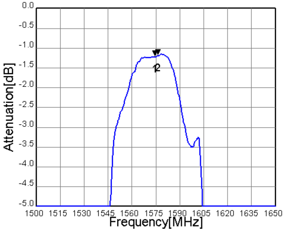
Fig.3 In-band Characteristic
