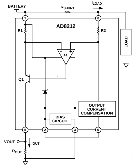
Figure 22. Typical Connection (7 V to 65 V Supply (Pin V+) Range)
