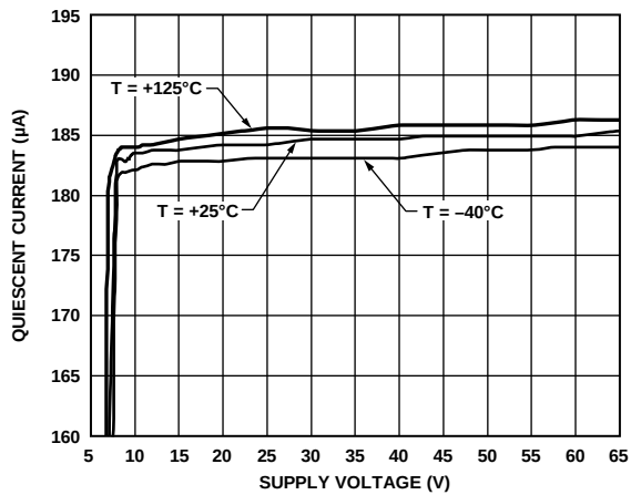
Figure 4. Supply Current vs. Supply (Pin V+) ( I_{OUT} = 0 mA)
