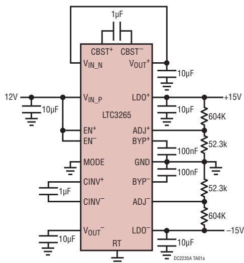
Low Noise \pm 15\text{V} Outputs from a Single 12V Input
