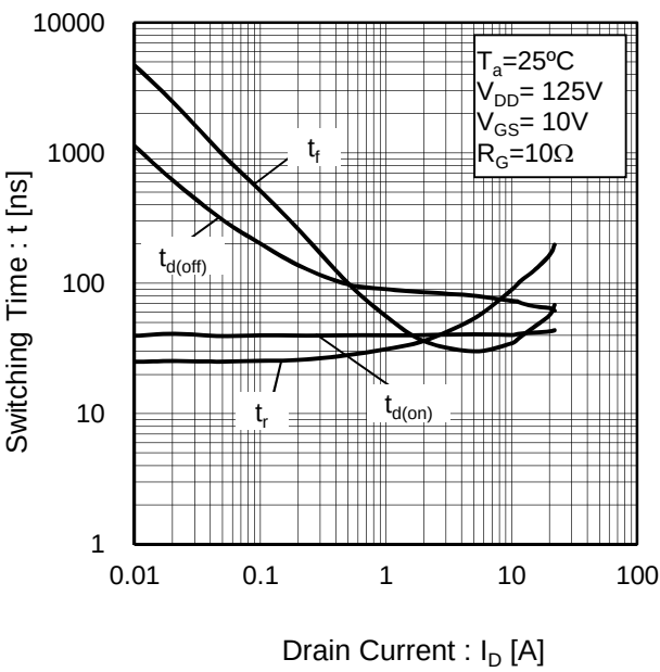
Fig.18 Switching Characteristics
