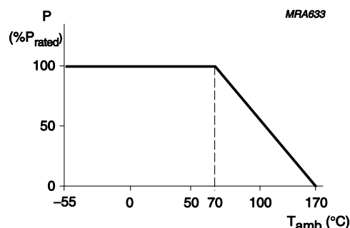
Fig. 5 Maximum dissipation ( P_{\max} ) in percentage of rated power as a function of the operating ambient temperature ( T_{\text{amb}} )
