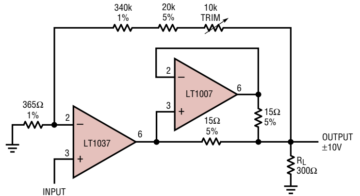
Precision Amplifier Drives 300 \Omega Load to \pm 10V
