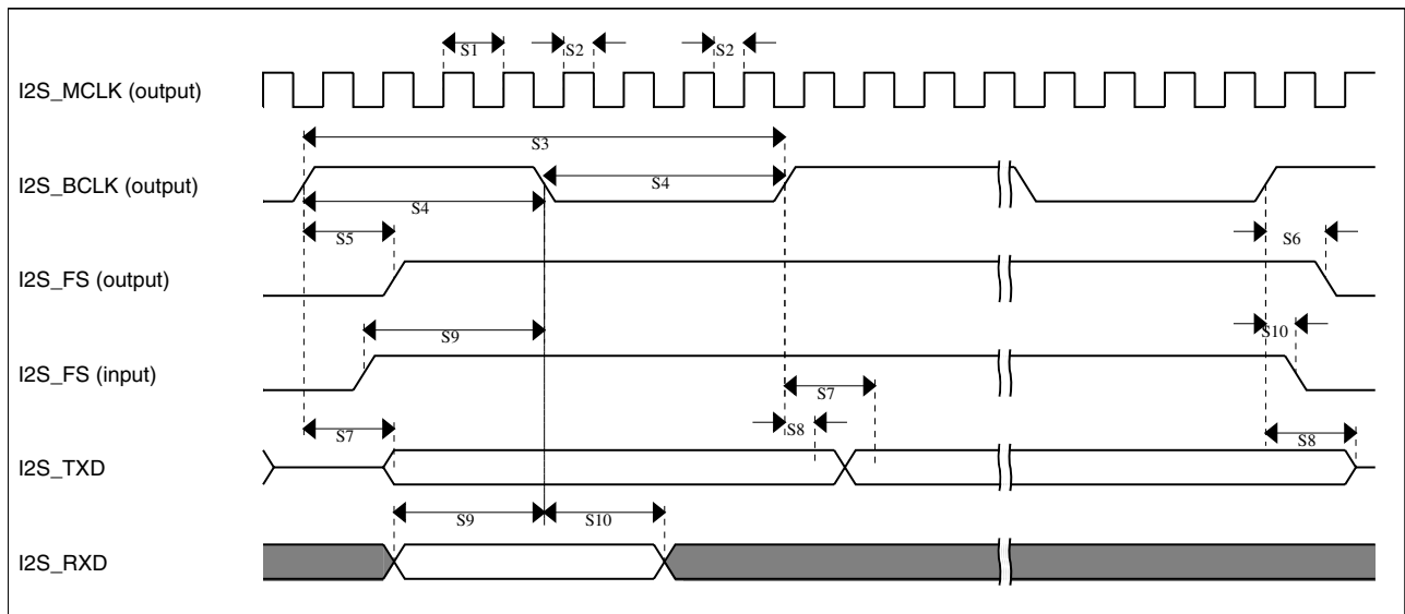
Figure 27. I²S timing — master mode
