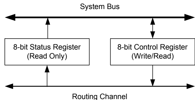
Figure 7-6. Status and Control Registers
