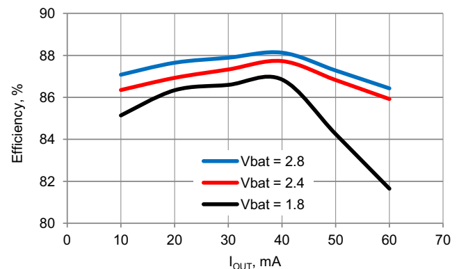
Figure 11-9. Efficiency vs I_{\text{OUT}} V_{\text{BOOST}} = 3.3 \text{ V} , L_{\text{BOOST}} = 22 \mu\text{H} [27]
