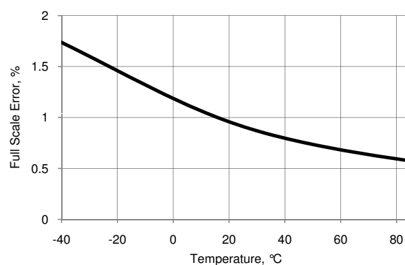
Figure 11-54. VDAC Full Scale Error vs Temperature, 4 V Mode
