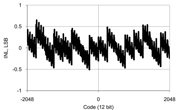
Figure 11-30. SAR ADC INL vs Output Code, Bypassed Internal Reference Mode
