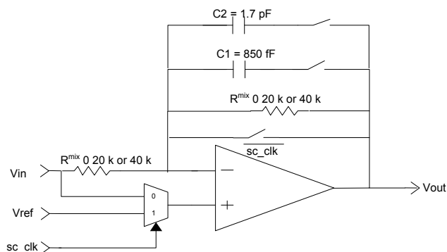
Figure 8-11. Mixer Configuration
