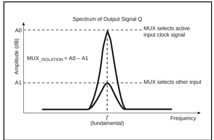
MUX Isolation
