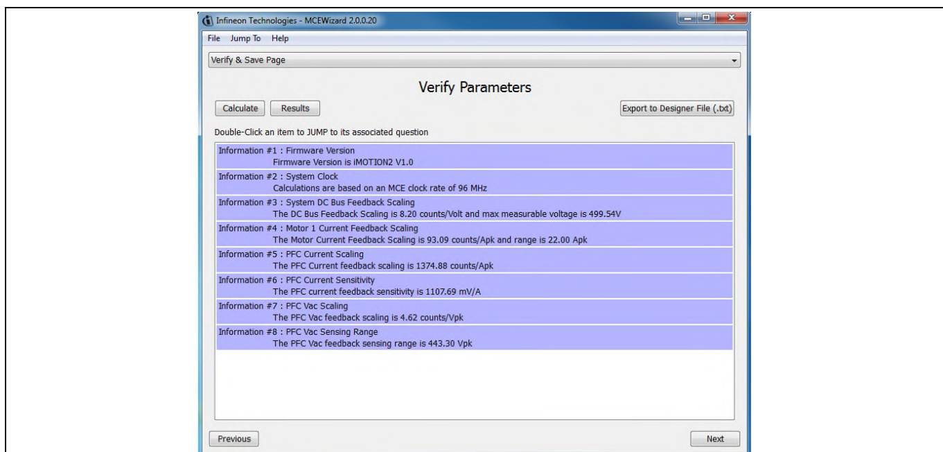
Figure 6 Verify and Save page for MCEWizard
