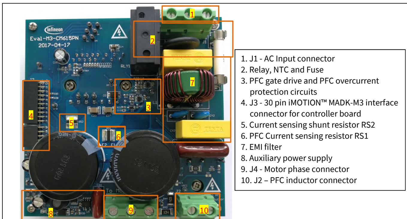
Figure 2 Functional groups of the Eval-M3-CM615PN evaluation board's top side
