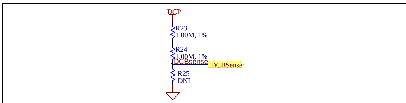
Figure 19 DC bus sense resistor on Eval-M3-CM615PN evaluation board
