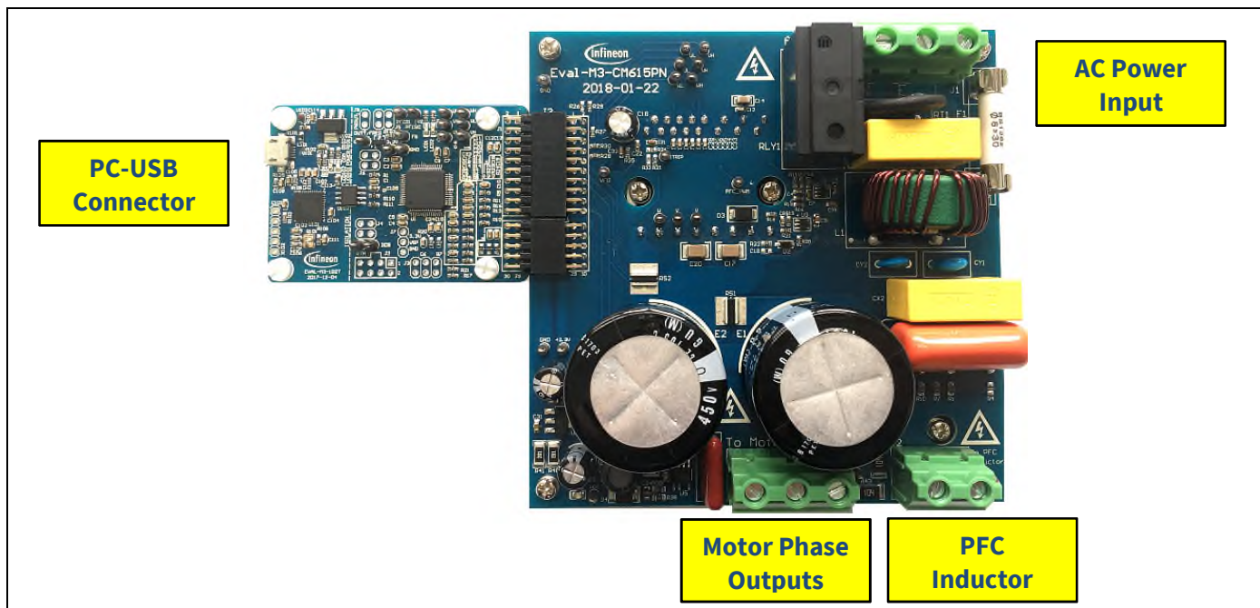
Figure 4 System connection example using EVAL-M3-CM615PN and EVAL-M3-102T
