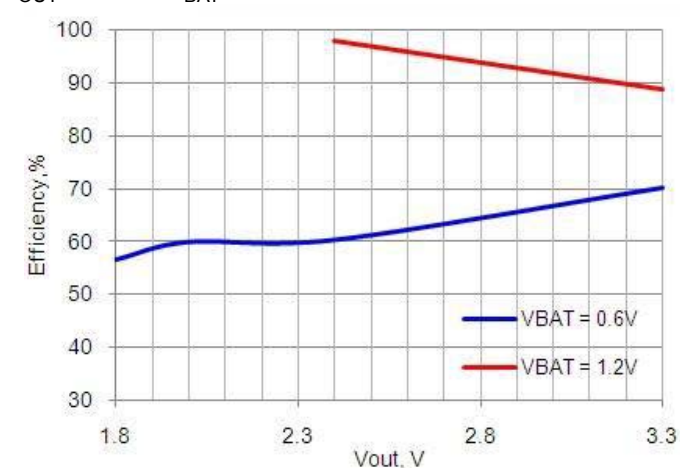
Figure 11-10. Efficiency vs V_{OUT}
