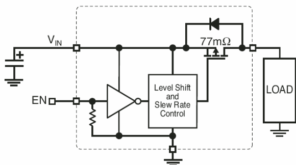
½ MIC94066, 68 Load Switch Application
