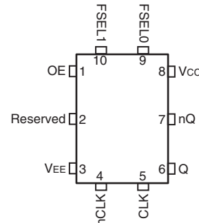
ICS8N3PG10MBKI-062 10-Lead VFQFN 5mm x 7mm x 1mm package body K Package Top View
