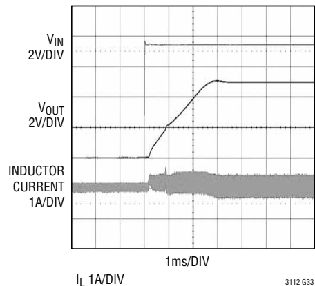
7.5V IN to 5.0V OUT Soft-Start Waveforms
