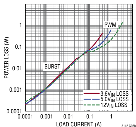
Wide V_{IN} to 12V OUT Power Loss
