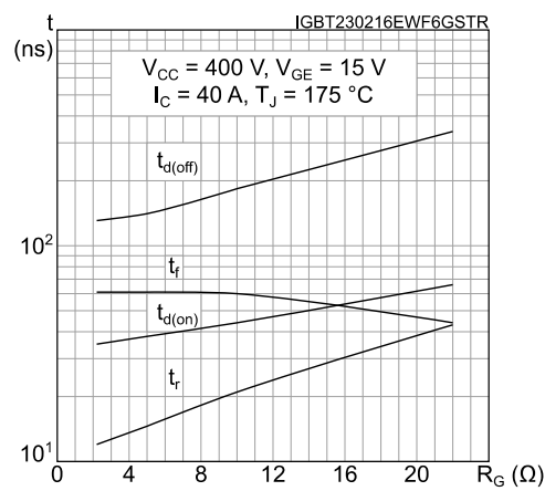
Figure 24: Switching times vs. gate resistance
