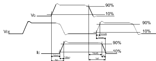
Figure 29: Switching waveform
