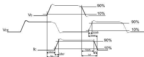
Figure 29: Switching waveform
