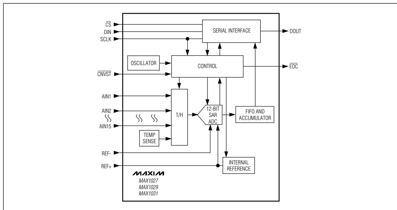
Figure 2. Functional Diagram
