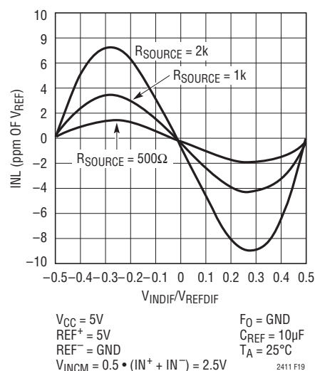
Figure 19. INL vs Differential Input Voltage ( V_{IN} = IN^+ = IN^- ) and Reference Source Resistance ( R_{SOURCE} at REF^+ and REF^- ) for Large C_{REF} Values ( C_{REF} \geq 1\mu\text{F} )
