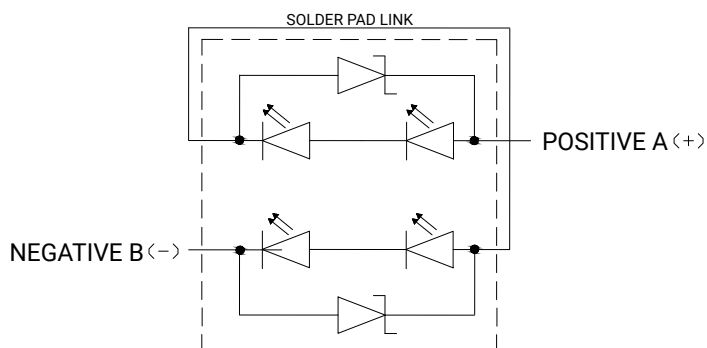
12-V Configuration
