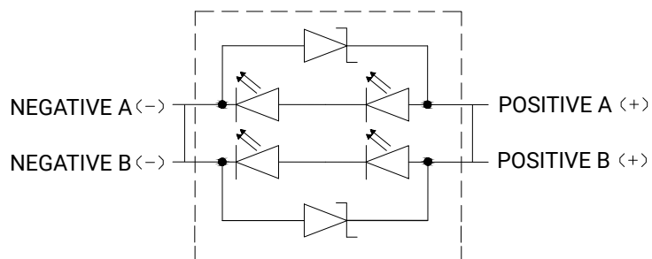
6-V Configuration
