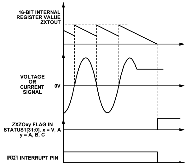
Figure 53. Zero-Crossing Timeout Detection
