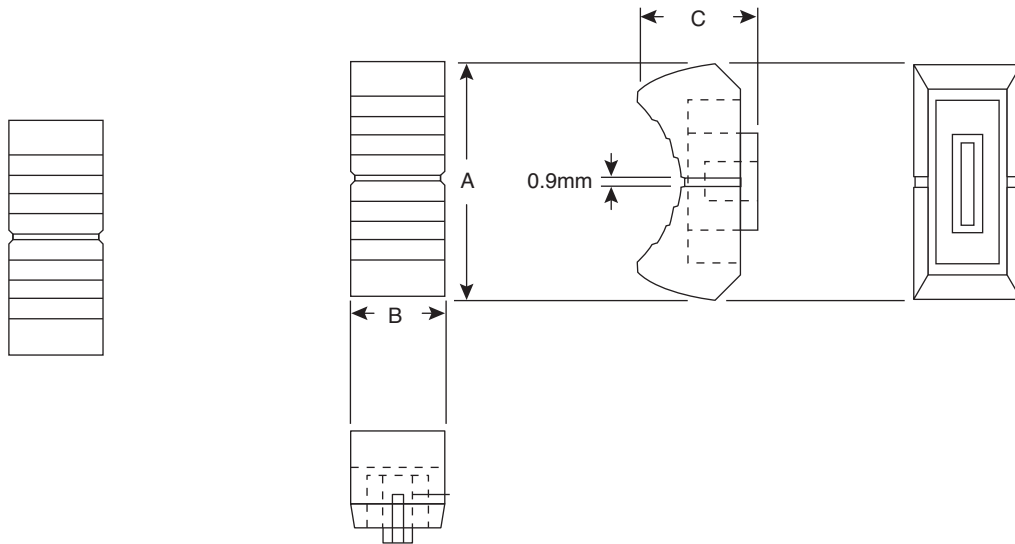
Dimensions: mm (in.)
