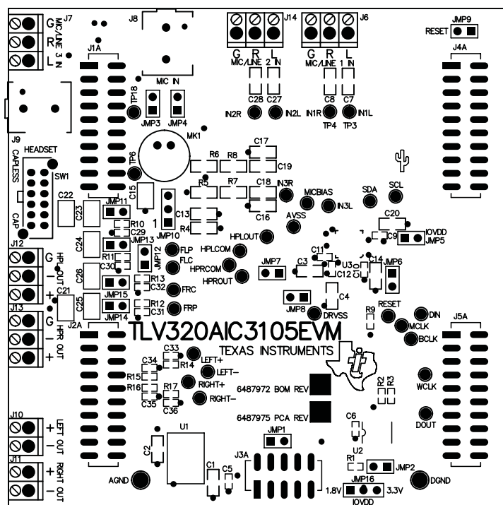
Figure C-1. Assembly layer
