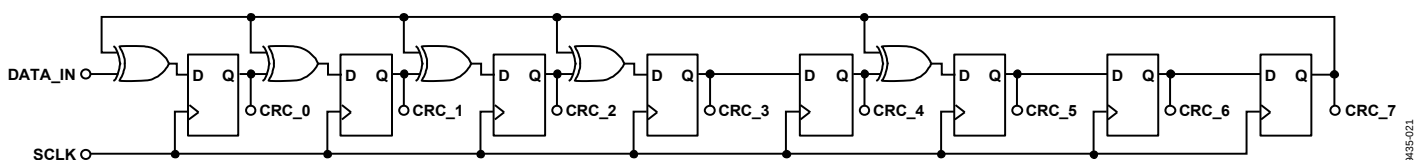
Figure 40. CRC Implementation
