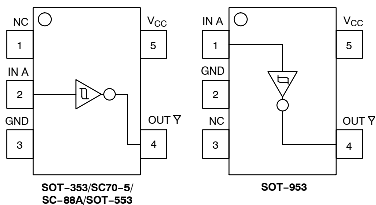
Figure 1. Pinout
