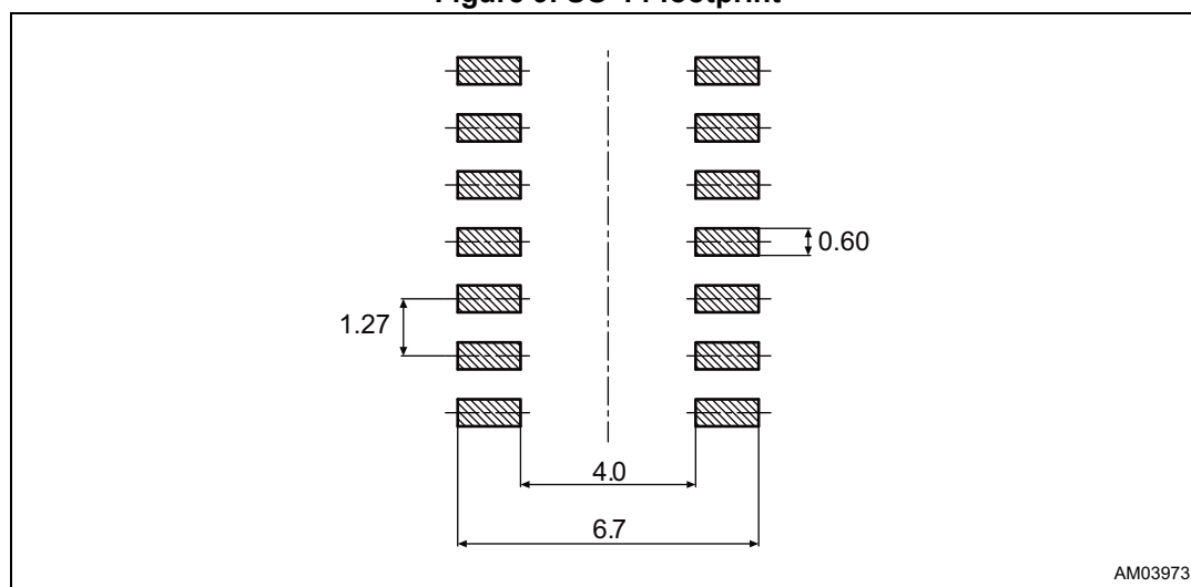
Figure 9. SO-14 footprint
