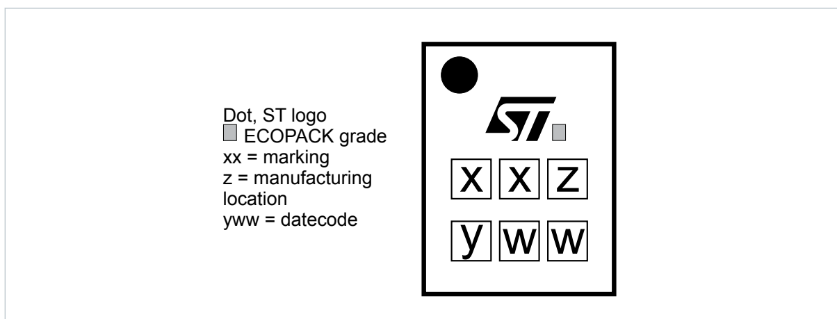
Figure 10. Marking
