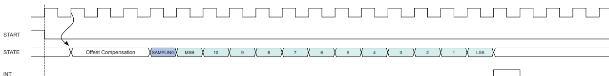
Figure 41-5. ADC Timing for One Conversion with Offset Compensation, 12-bit
