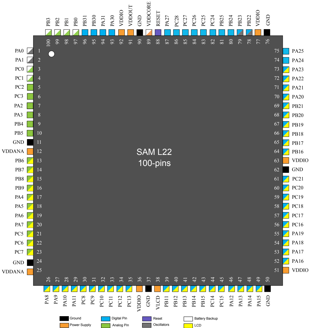
Figure 5-3. TQFP100
