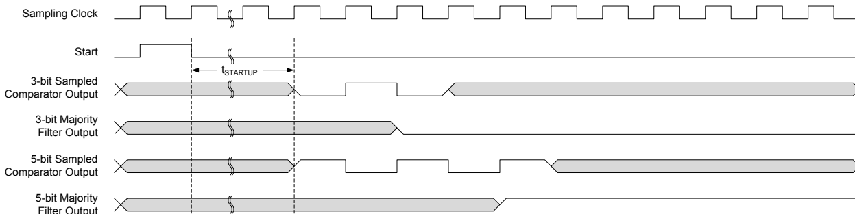
Figure 42-7. Single-Shot Filtering
