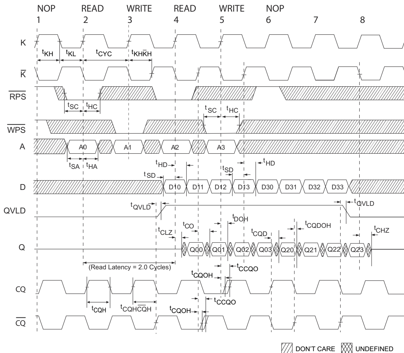
Figure 6. Waveform for 2.0 Cycle Read Latency [39, 40, 41]
