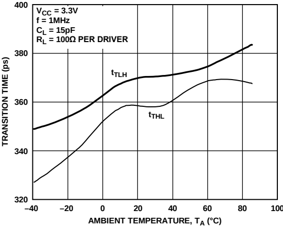
Figure 23. Transition Time vs. Ambient Temperature
