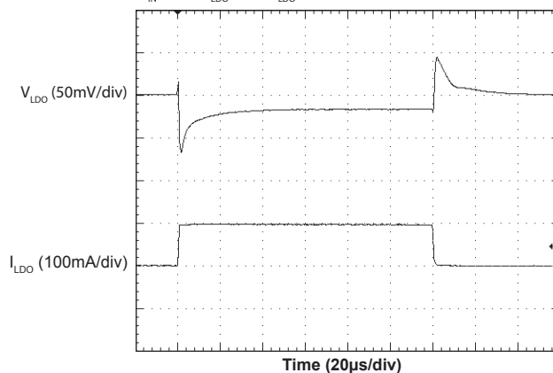
LDO Load Transient Response (3.3V)
