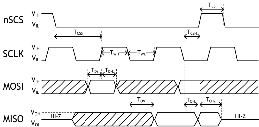
Figure 24 SPI Timing
