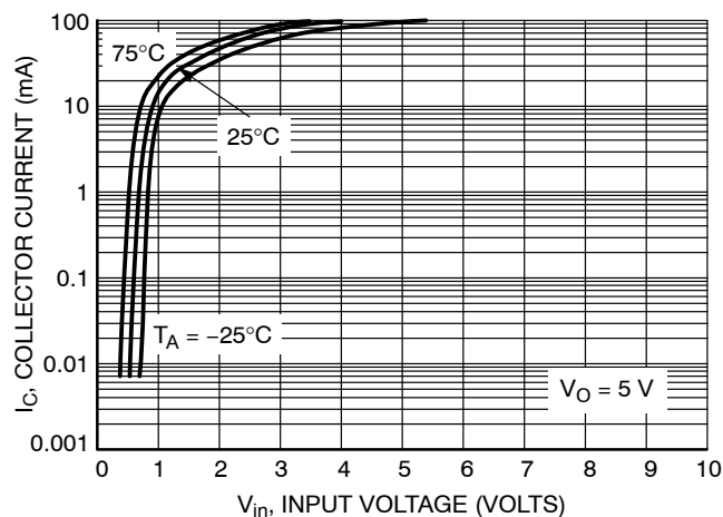
Figure 99. Output Current versus Input Voltage
