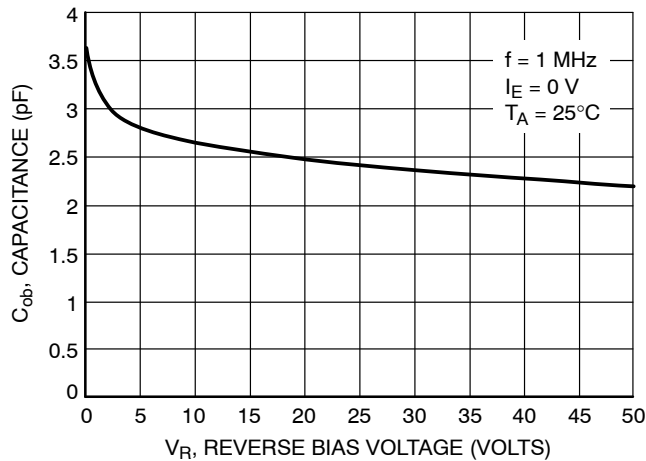
Figure 93. Output Capacitance
