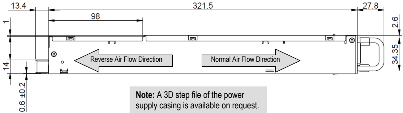
Figure 41: Side view 1
