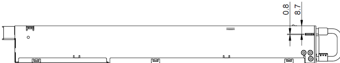
Figure 43: Side view 2
