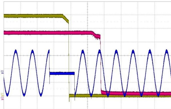
Figure 12: AC drop out 30 ms (20 ms/div) CH1: V_1 (2 V/div) CH2: V_{SB} (1 V/div) CH3: V_{in} (200 V/div)
