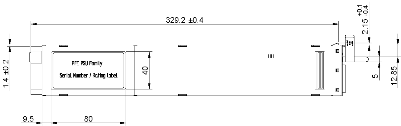
Figure 42: Top view
