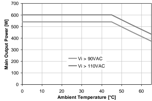
Figure 40: Thermal derating for PFE600-12-054RA
