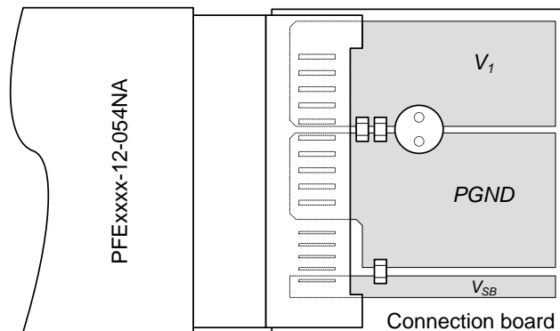
Figure 5: Output ripple test setup
