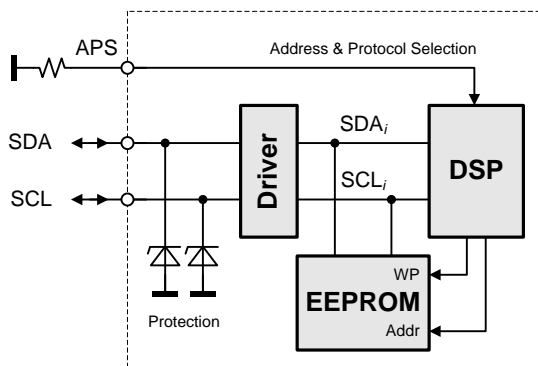
Figure 35: I 2 C Bus to DSP and EEPROM
