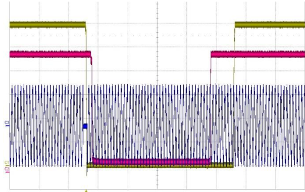
Figure 13: AC drop out 30 ms (200 ms/div), V_1 restart after 1 sec CH1: V_1 (2 V/div) CH2: V_{SB} (1 V/div) CH3: I_1 (200 V/div)
