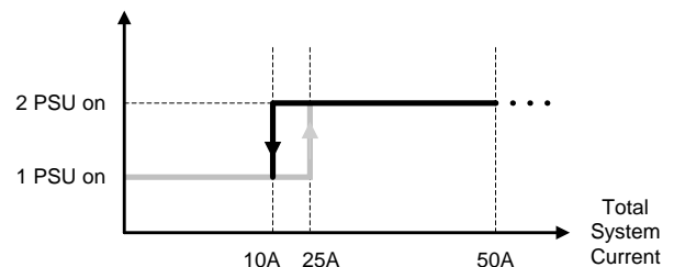
Figure 29: Hot-standby enable/disable current thresholds
