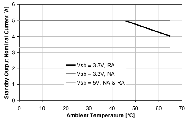
Figure 22: Temperature derating on V_{SB}
