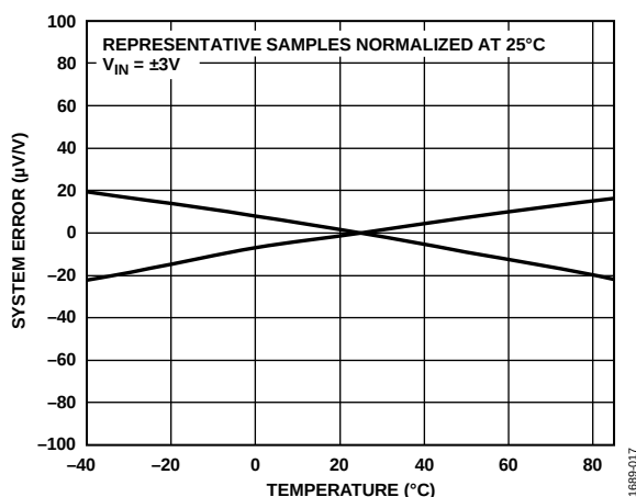
Figure 17. System Error vs. Temperature, Normalized at 25°C
