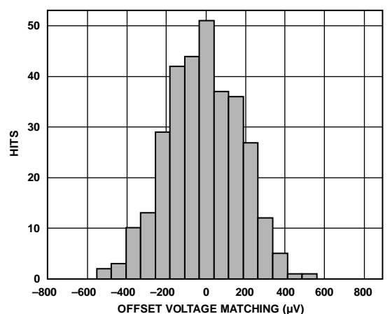
Figure 7. Typical Distribution of Offset Voltage Matching
