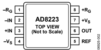
Figure 2. Pin Configuration
