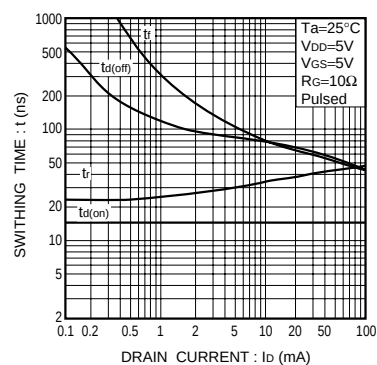
Fig.20 Switching characteristics
