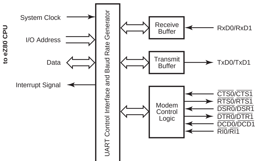
Figure 36. UART Block Diagram
