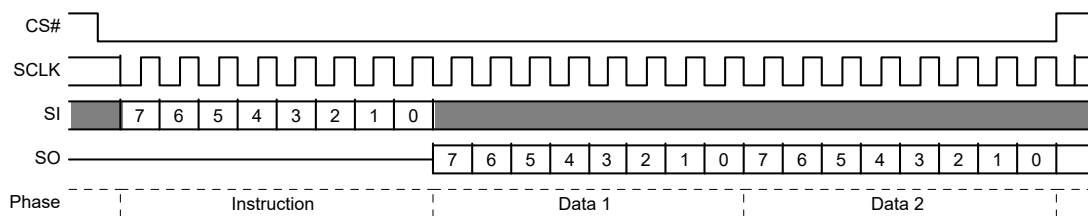
Figure 15. Single Bit Wide Output Command without Latency
