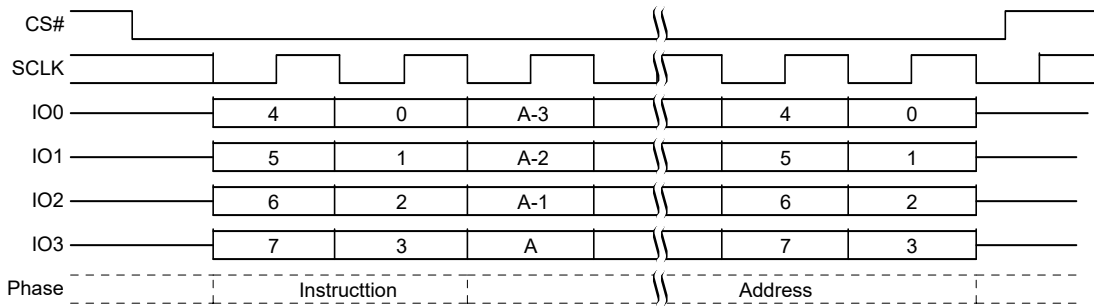
Figure 83. Half Block Erase (HBE 52h or 4HBE 53h) QPI Mode Command Sequence
