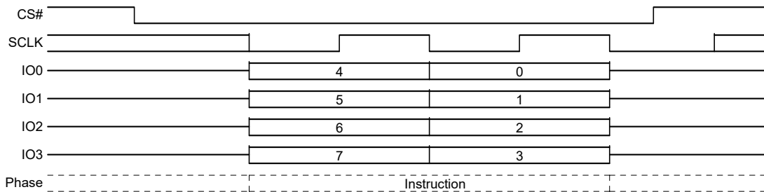
Figure 58. Exit 4 Byte Address QPI Mode
