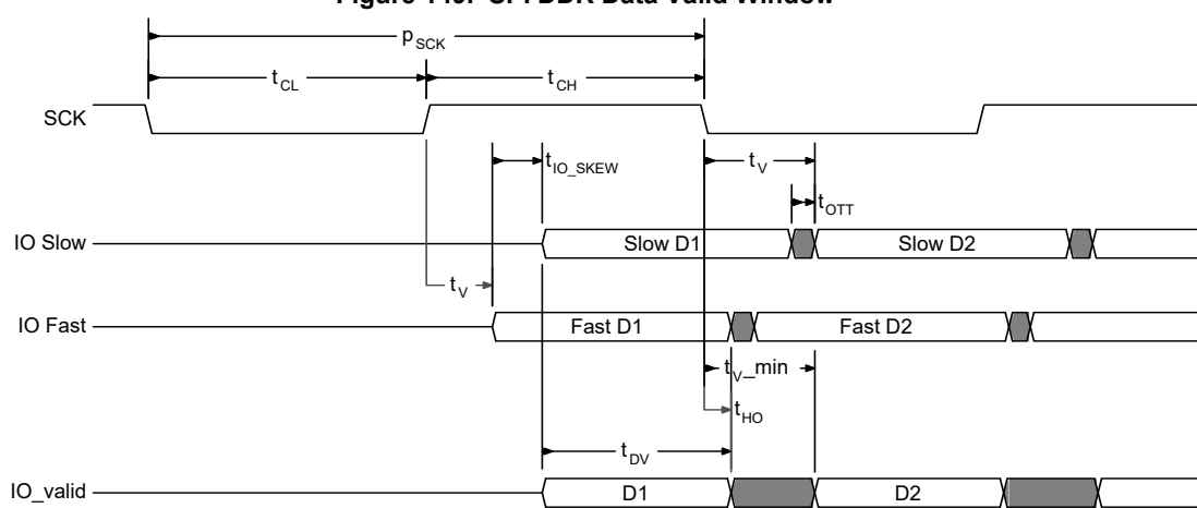
Figure 149. SPI DDR Data Valid Window
