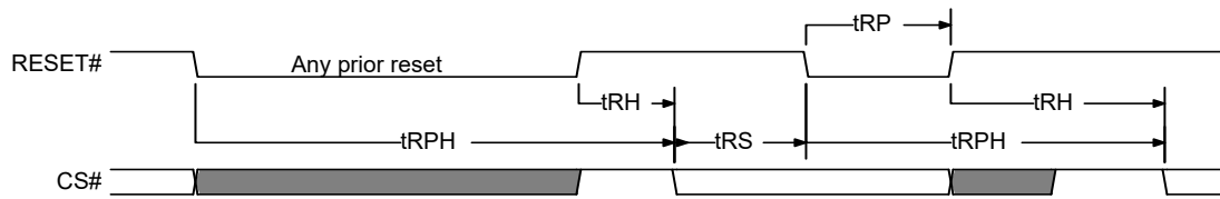
Figure 139. Hardware Reset using RESET# Input
