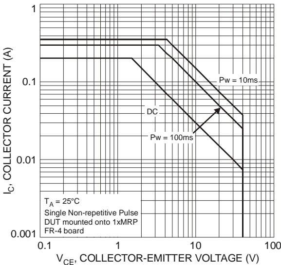
Fig. 5 Typical Collector Current vs. Collector-Emitter Voltage
